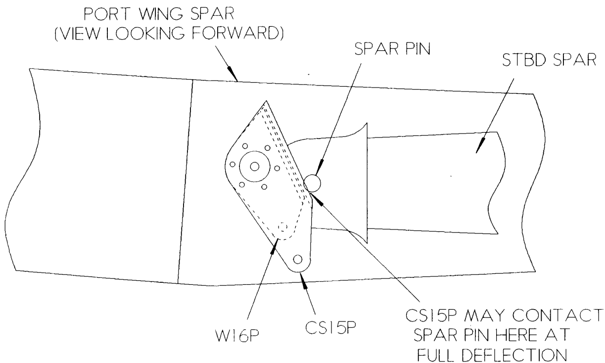
Fig 4. Detail of port side aileron quick connect bellcrank.
