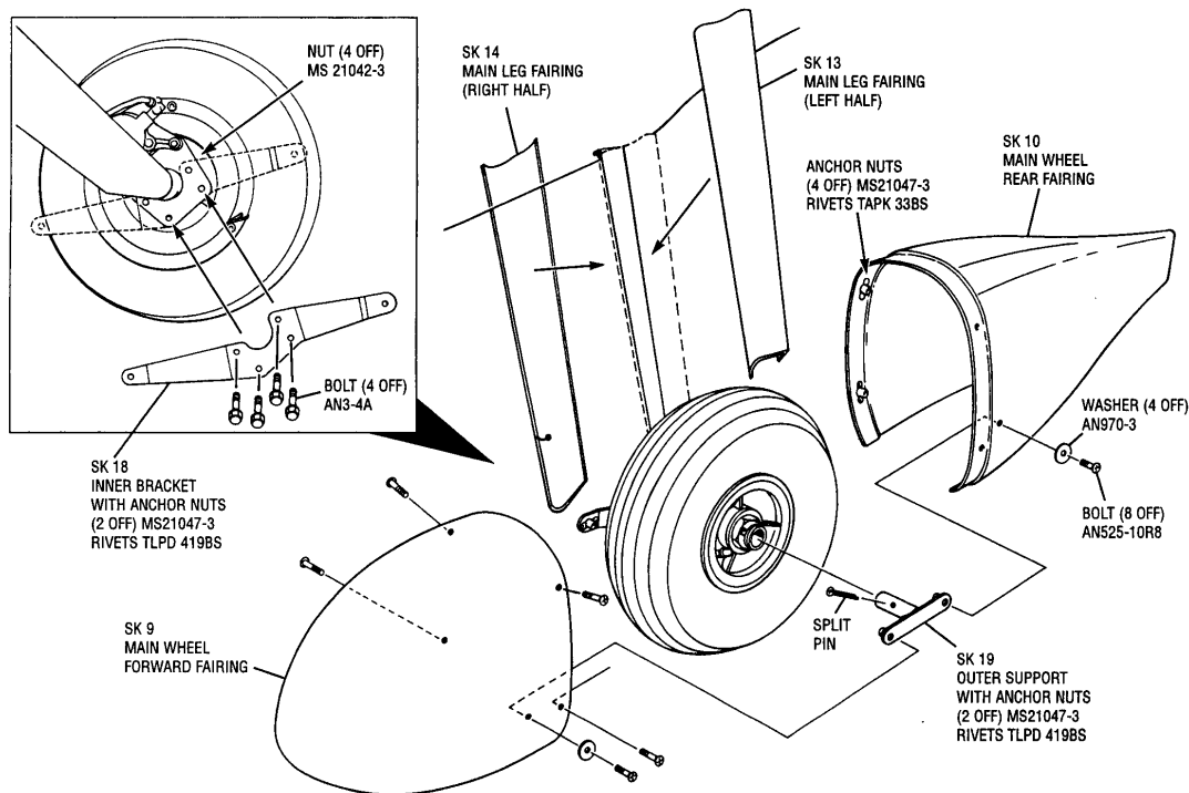
Fig 3. Main Gear Fairings (Port side shown)
