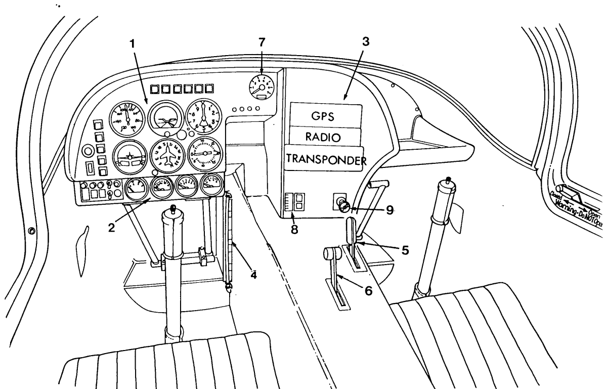
Figure 1 - 1 Cockpit Layout
