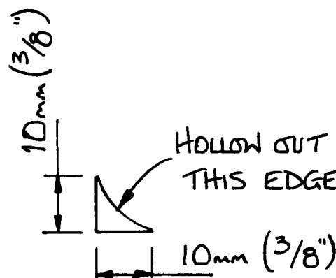
Stall strip section. Make two from wood 23cm (9") long
