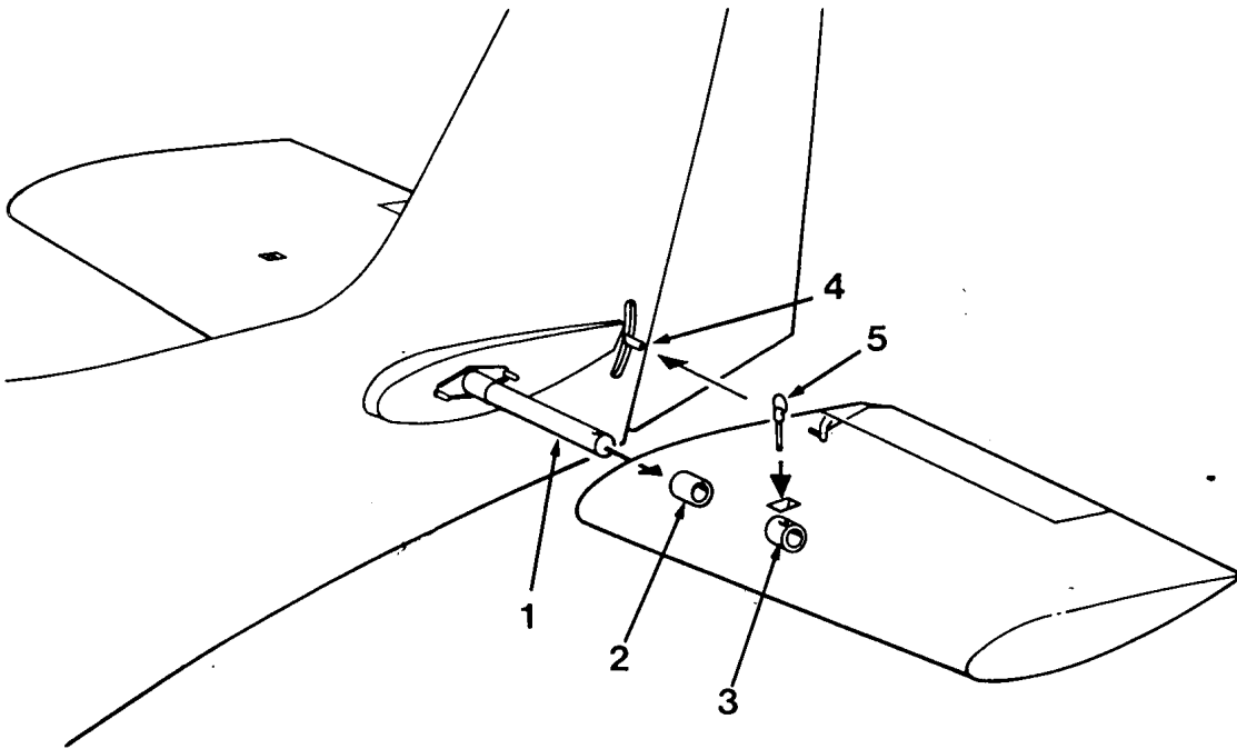
Fig 2. Tailplane rigging.
