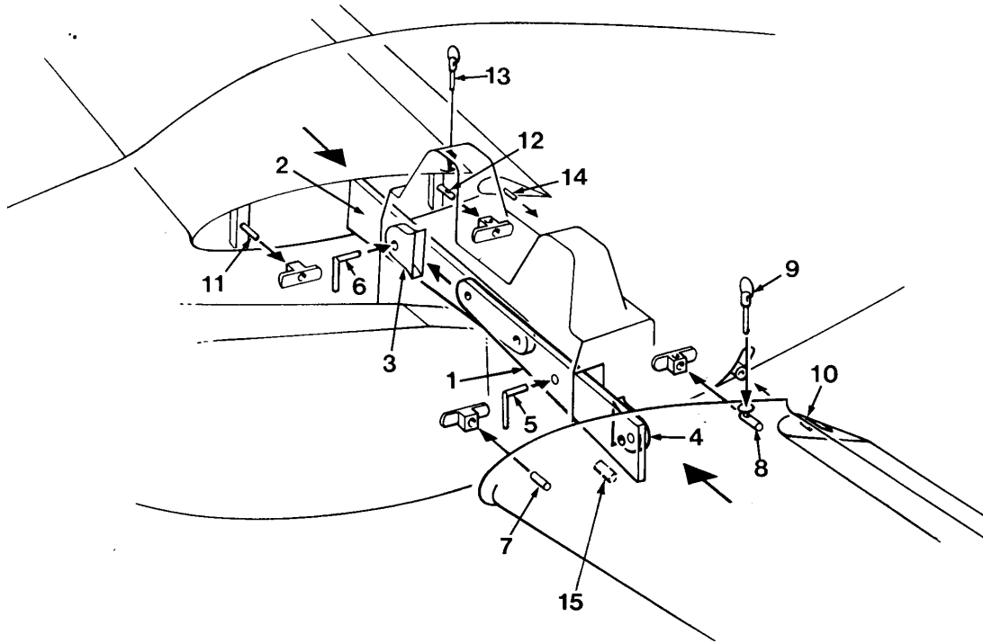
Fig 1. Wing rigging.
